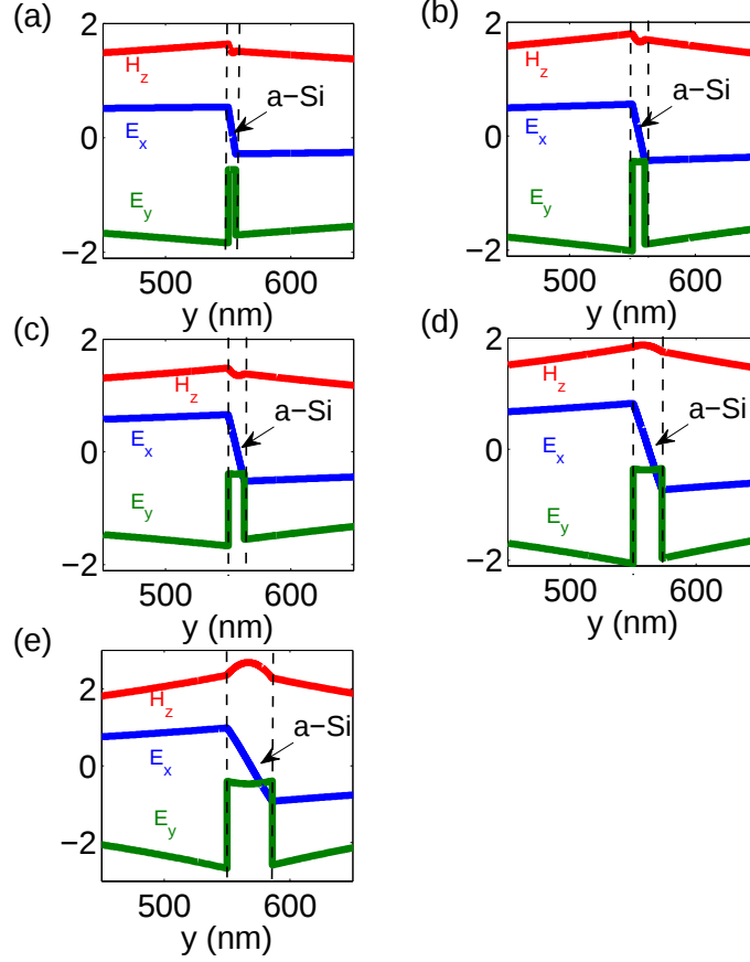
Figure 5.8: Transverse and longitudinal components of the electric and magnetic field of guided modes on thin layer of a-Si with a thickness of (a) 6 nm, (b) 10 nm, (c) 13 nm, (d) 23 nm, and (e) 36 nm surrounded by SiO 2 .
