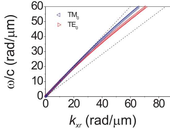
Figure 2.7: Dispersion relation of the two fundamental ( m = 0 ) \text{TM}_0 and \text{TE}_0 waveguide modes. The represented multilayers structures are a 30 nm slab \epsilon_2 = 2 + 0.01i surrounded by air \epsilon_{1,3} = 1 . The dashed lines represents the light line in air and slab.
