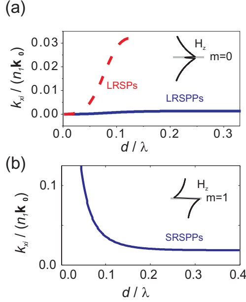
Figure 2.9: (a) Imaginary components of the complex wave number, k_x = k_{xr} + i k_{xi} , of long-range and (b) short-range surface modes in thin films of materials with \epsilon_2 = -20 + 1i and \epsilon_2 = 1 + 20i surrounded by air. k_{xi} are normalized to n_1 k_0 and are displayed as a function of the thickness of the layer normalized by the wavelength at \lambda = 600 nm. The inset of (a) and (b) are the field distribution for the symmetric (long-range) and antisymmetric (short-range) modes.
