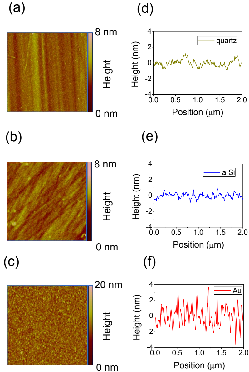
Figure 4.2: AFM images of a \text{SiO}_2 substrate (a), an amorphous silicon thin film with a thickness of 13 nm on top of a \text{SiO}_2 substrate (b), and (c), a gold layer of a thickness of 44.2 nm on top of BK7 substrate with 3 nm of Ti for adhesion purposes. The gold layer is purchased from Biacore [83] and it is a standard substrate for surface plasmon resonance sensors. (d),(e)(f) are line scans of the \text{SiO}_2 , amorphous silicon and gold AFM images, which lead to R_q the measured surface roughness.
