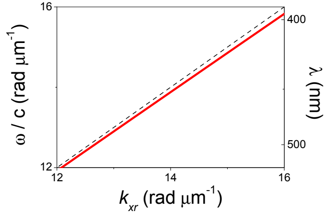
Figure 1.2: Dispersion curve, i.e., frequency versus the real component of the wave number along the propagation direction of a long-range surface polariton in a thin film ( d = 20 \text{ nm} ) of a material with permittivity \epsilon_2 = 1 + 20i surrounded by vacuum. The dashed line indicates the edge of the light cone.
