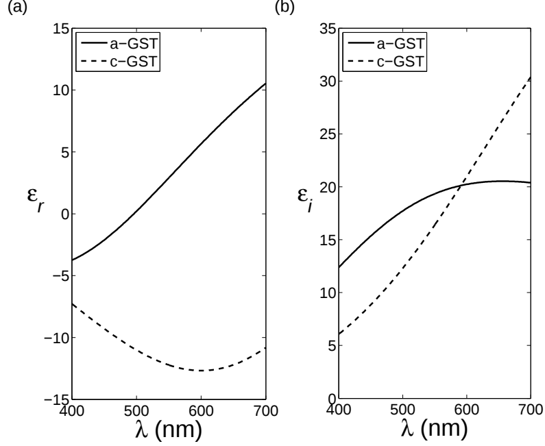
Figure 3.1: Permittivity of \text{Ge}_{17}\text{Sb}_{76}\text{Te}_7 . The solid lines correspond to the amorphous phase and the dashed lines to the crystalline phase. Figure (a) displays the real component of the permittivity, while (b) shows the imaginary component.
