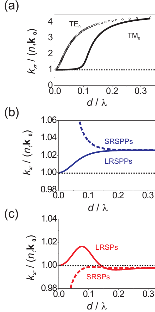
Figure 2.8: Real component of the complex wave number k_x = k_{xr} + ik_{xi} , normalized to n_1 k_0 , of guided modes in a thin slabs with (a) \epsilon_2 = 20 + 1i , (b) \epsilon_2 = -20 + 1i and (c) \epsilon_2 = 1 + 20i and surrounded by air as a function of the thickness of the layer normalized by the wavelength at \lambda = 600 nm. The dashed line in (b) and (c) indicates the light line in air, n_1 = 1 .
