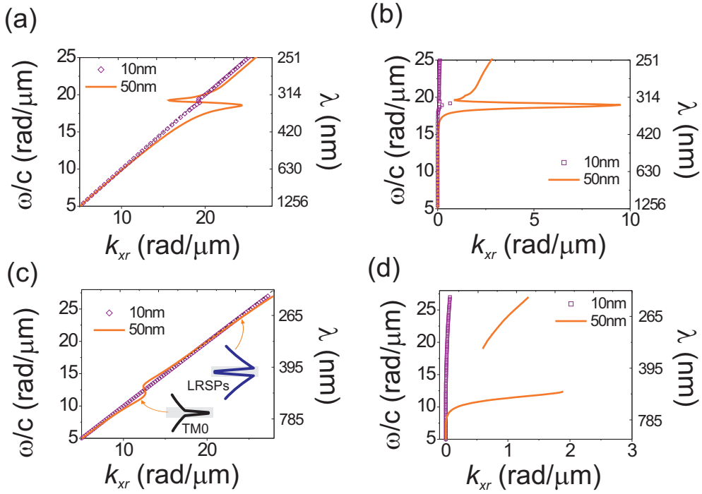
Figure 2.12: (a),(b) Dispersion of long-range Surface plasmon polaritons at the interface of a silver thin layer with air. (c),(d) Dispersion of long-range guided modes at the interface of a amorphous silicon thin layer with air. The thicknesses of the thin layer are chosen for 10 and 50 nm. The dashed line corresponds to the light line in air, \omega/c = \sqrt{\epsilon_1} k_0 . The inset shows the magnetic field component of H_z for the case of 50 nm a-Si supporting TM_0 mode at 600 nm and LRSPs mode at 300 nm.
