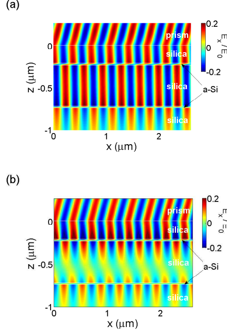
Figure 7.4: Color plot of the electric field component along the x-direction in the x-z plane direction of the a-Si multilayer displayed in Fig. 7.1 calculated for \lambda = 520 nm and an angle of incidence of (a) \theta = 65.4^\circ and (b) \theta = 67.4^\circ .
