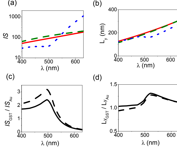
Figure 6.9: (a), Calculated intrinsic sensitivity and (b), decay length of LRSPs for a film with a thickness d of 20 nm of Au (dotted curve), c-GST (dashed curve) and a-GST (solid line) as a function of the wavelength. Intrinsic sensitivity (c), and decay length (d), ratio between a film of a-GST (c-GST) and Au, solid (dashed) curves, as a function of the wavelength. For all the calculations, the thin film is surrounded by a medium with a refractive index of 1.33.
